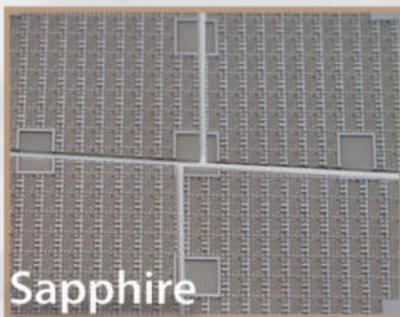
Decapsulated Die
